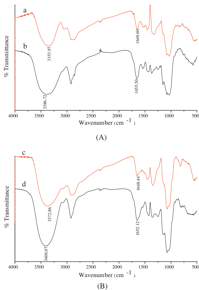
Fig. 1. Infrared spectra of BiHEP25 (a), HEP25 (b), BiHEP75 (c), and HEP75 (d) in the frequency range of 500–4000 cm -1 .
